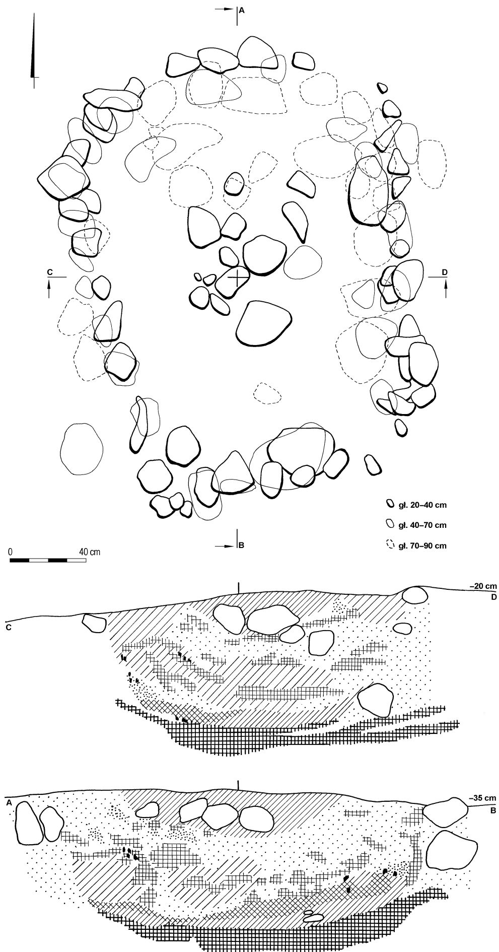
Ryc. 10. Łęgonice, pow. Grójec, stan. 1. Plan i profile pieca Fig. 10. Łęgonice, distr. Grójec, site 1. Plan and cross-section of the oven
