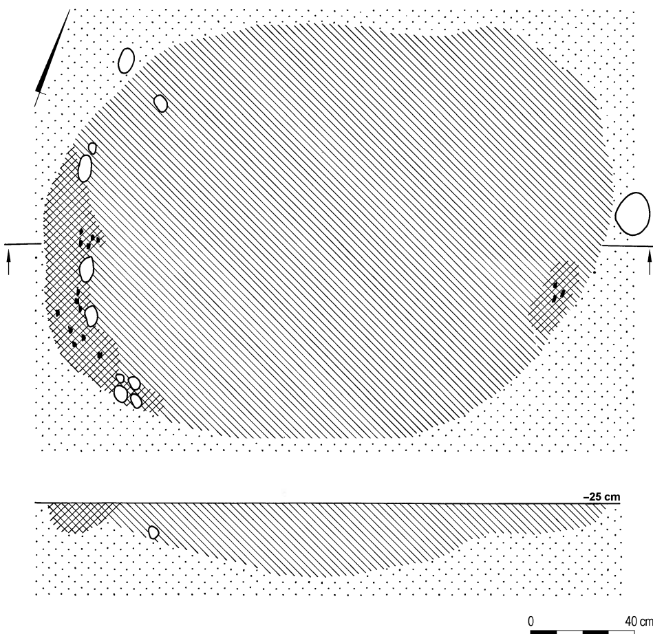
Ryc. 21. Łęgonice, pow. Grójec, stan. 1. Plan i profil jamy 5. Fig. 21. Łęgonice, distr. Grójec, site 1. Plan and cross-section of pit 5
