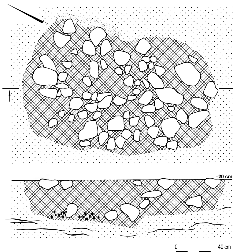
Ryc. 12. Łęgonice, pow. Grójec, stan. 1. Plan i profil paleniska 3 Fig. 12. Łęgonice, distr. Grójec, site 1. Plan and cross-section of hearth 3
